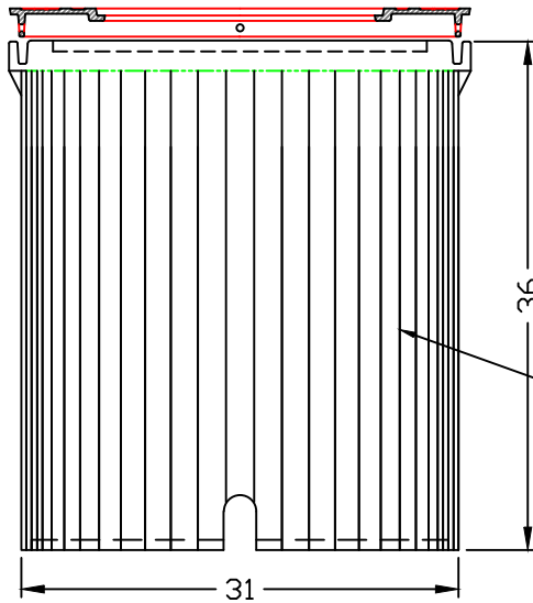
CRUSH RESISTANT RIBBING DFW2836FD
