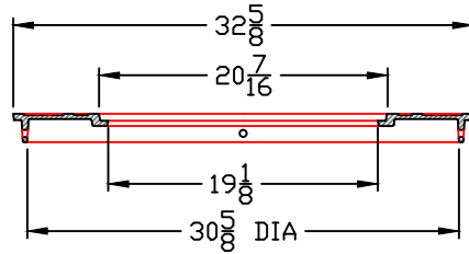
RING SECTION
